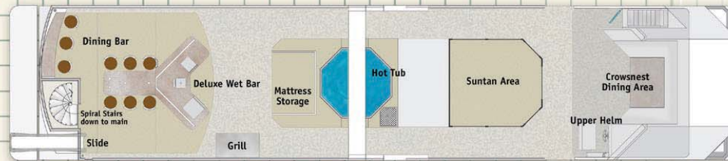
BRIDGE DECK
